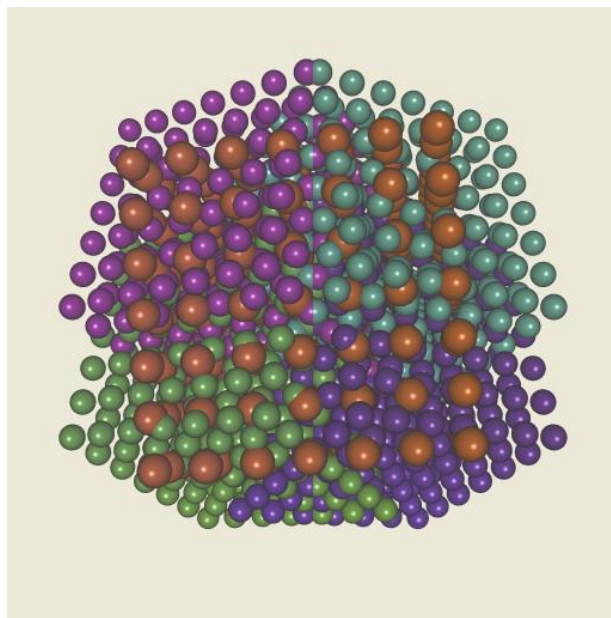
Fig. 1. Molecular structures
