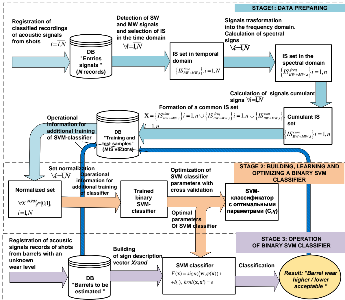
Fig. 6. General scheme of information technology for technical diagnostics of the state of barrels by a set of informative signs
