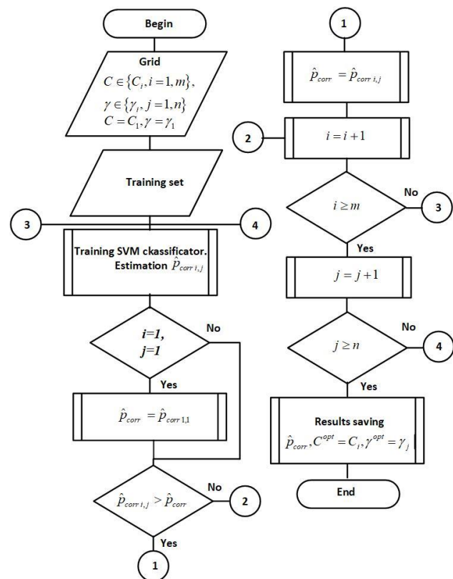
Fig. 4. Block diagram of the cross-validation algorithm for choosing the optimal hyperparameters
