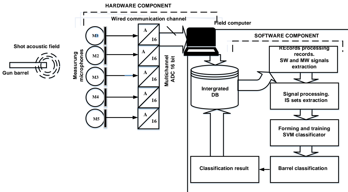
Fig. 7. Automated system for technical diagnostics of barrels' condition based on a set of informative signs
