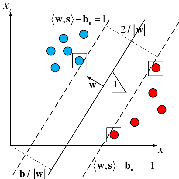
Fig. 2. Graphical representation of the SVM classifier in two-dimensional space Source: compiled by the author
