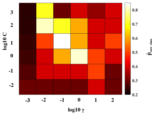
Fig. 5. The result of the first stage of selection of hyperparameters C and \gamma Source: compiled by the author
