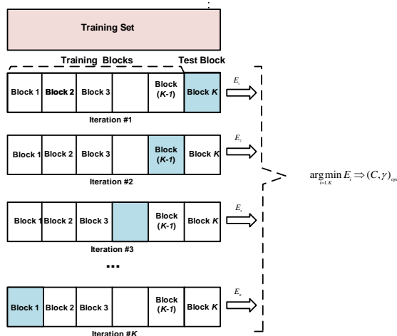
Fig. 3. Scheme of hyperparameters optimization by the cross-validation method
