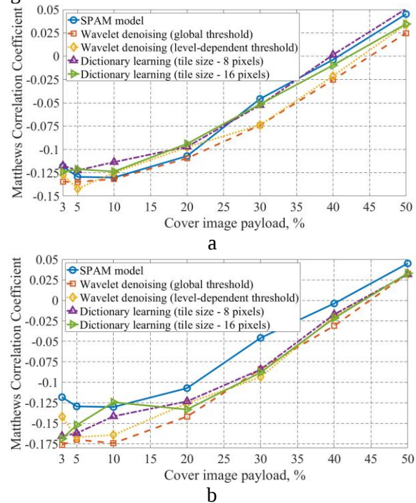
Fig. 3. The dependency of Matthews Correlation Coefficient on cover image payload for stego images generated by HUGO embedding method and usage of F_{DF} (a) and F_{CC} (b) features for F_a=0\% and applying of spectral calibration methods
