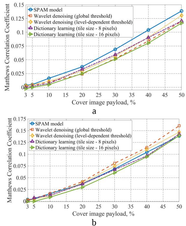
Fig. 1. The dependency of Matthews correlation coefficient on cover image payload for stego images generated by HUGO embedding method
