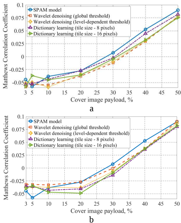
Fig. 2. The dependency of Matthews Correlation Coefficient on cover image payload for stego images generated by HUGO embedding method and usage of F_{DF} (a) and F_{CC} (b) features for
